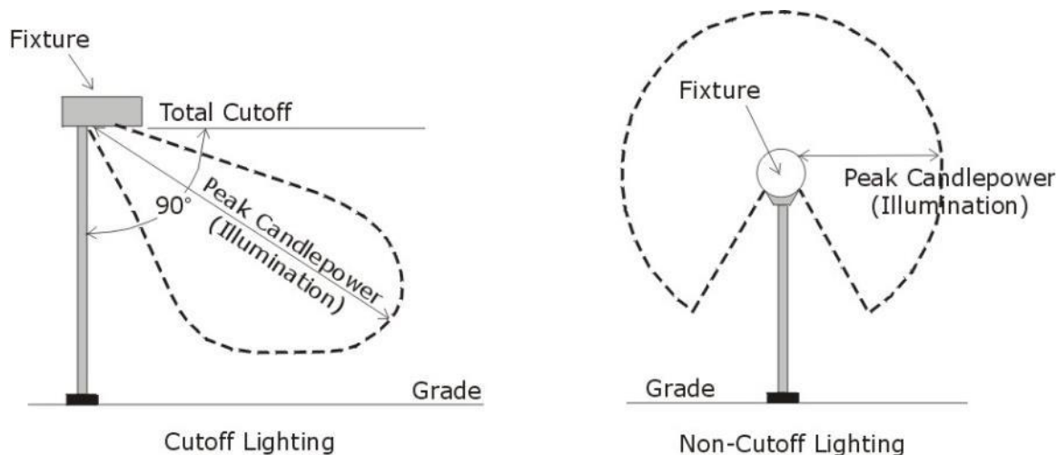
Figure 1109-A: Cutoff lighting fixtures (left) versus non-cutoff lighting fixtures (right).
