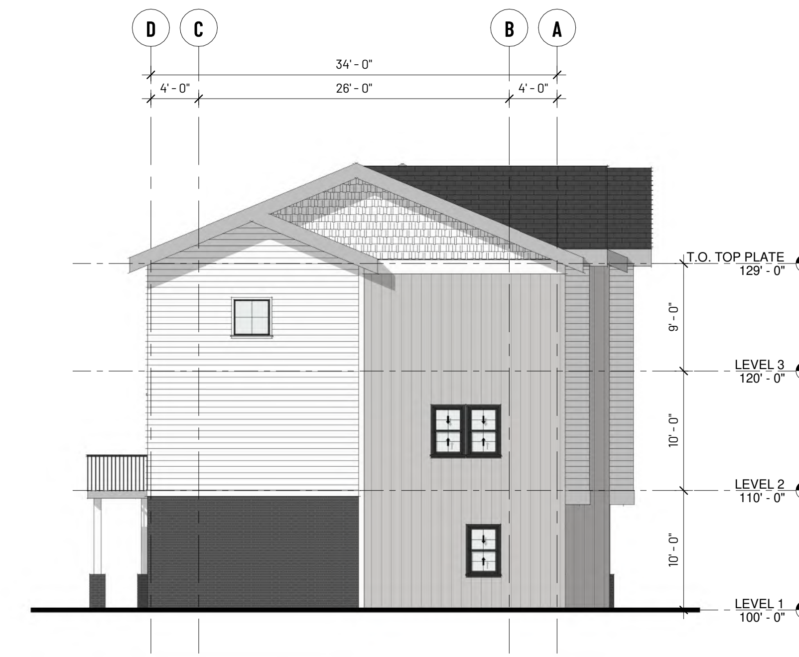
02 LEFT ELEVATION - 2 CAR GARAGE 1/8" = 1'-0"
