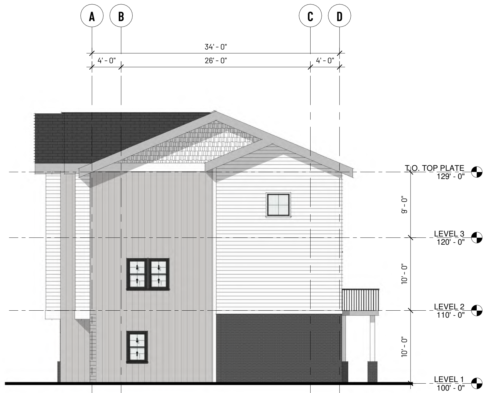
04 RIGHT ELEVATION - 2 CAR GARAGE 1/8" = 1'-0"
