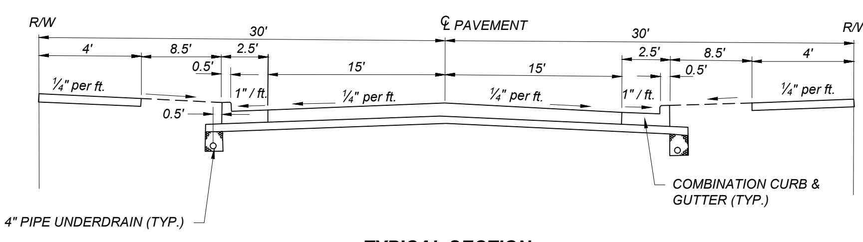
TYPICAL SECTION Not to Scale
